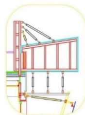
Figure 8: Cross section of the roof protector structure (http://archipaper.ir/category/cad/energy-arch)
