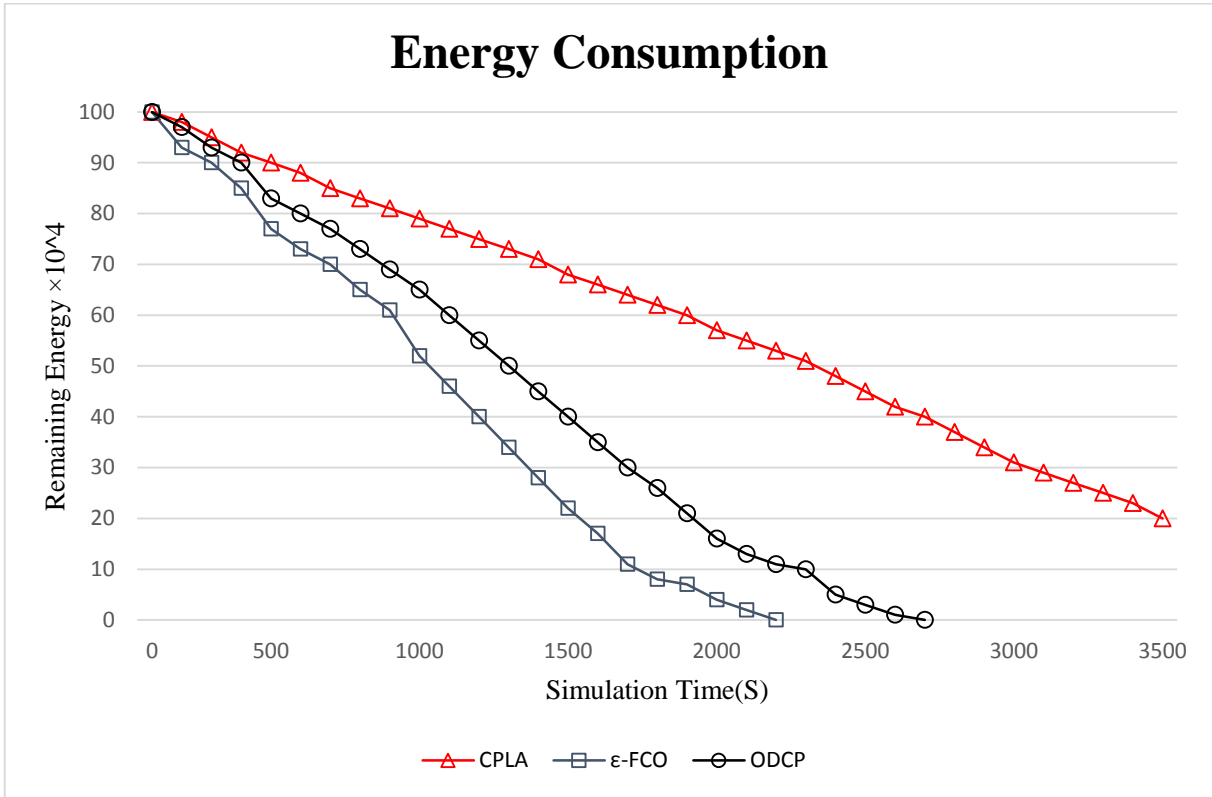
Figure 9- Testing energy consumption rate in CPLA network during activity, comparing to ODCP and ε-FCO protocols
